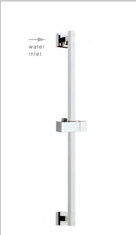
SR-4DWM Length:700mm Size:19X19mm Material:1/2 Brass
