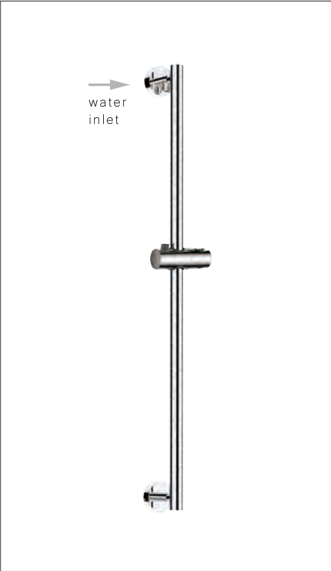
SR-3EWM Length:650mm Size:Φ24mm Material:Brass
